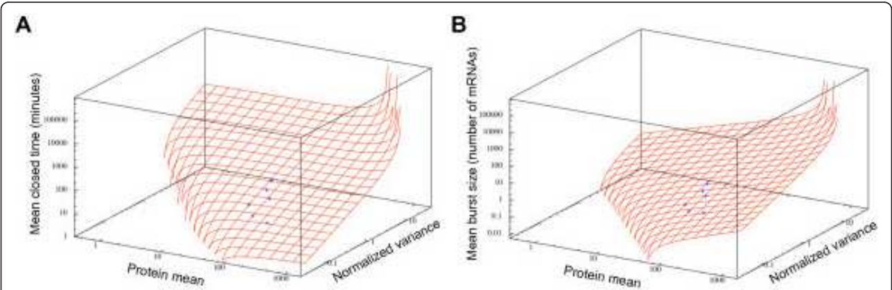
Figure 5 Inference of burst size and closed time from mean and normalized variance (NV) of protein levels. (A) At steady states, using the best transcription-translation parameter set ( \rho , \bar{\rho} , \gamma , \bar{\gamma} and \alpha ) and the modified Paulsson's equation system, the mean closed time could be calculated from the protein mean and protein NV (red grid). (B) Using the same data and equation system as in panel (A), the mean burst size could be calculated from the protein mean and protein normalized variance (red grid). Note that grids of both panels are linked because each value pair (protein mean and NV) corresponds to a single value pair (mean burst size and mean closed time). For both parts, clones C1, C3, C5, C7, C11, and C17 are represented as blue points on the grid, and all axes are on a logarithmic scale.
