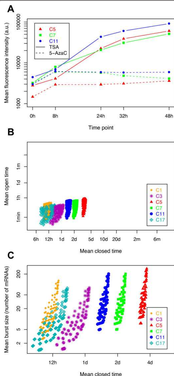
Figure 3 Exploration of model parameters based on treatments with chromatin-modifying agents. (A) Evolution of mean fluorescence intensity following kinetics of treatment with trichostatin A (TSA; solid line) and 5-azacytidine (5-AzaC; dotted line) (0 to 48 hours) for three cellular clones. (B) Distributions of the plausible chromatin dynamics. For each clone, all 114 possible couples of ( 1/k_{on} ; 1/k_{off} ) values were plotted, expressed as mean open time ( 1/k_{off} ) and mean closed time ( 1/k_{on} ), after removal of all parameter sets that were not able to account for the transcription-translation dynamics under TSA and 5-AzaC treatments. (C) This experiment was the same as for (B), except than the transcription rate ( \rho ) and the mean open time ( 1/k_{off} ) parameters were reduced to a single effective parameter ( \rho/k_{off} ), representing the mean burst size. min, minutes; h, hours; d, days; m, months.
