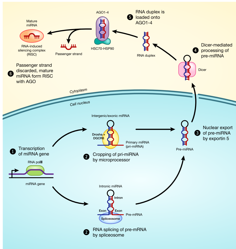
Fig. 1. Schematic model of miRNA biogenesis.
